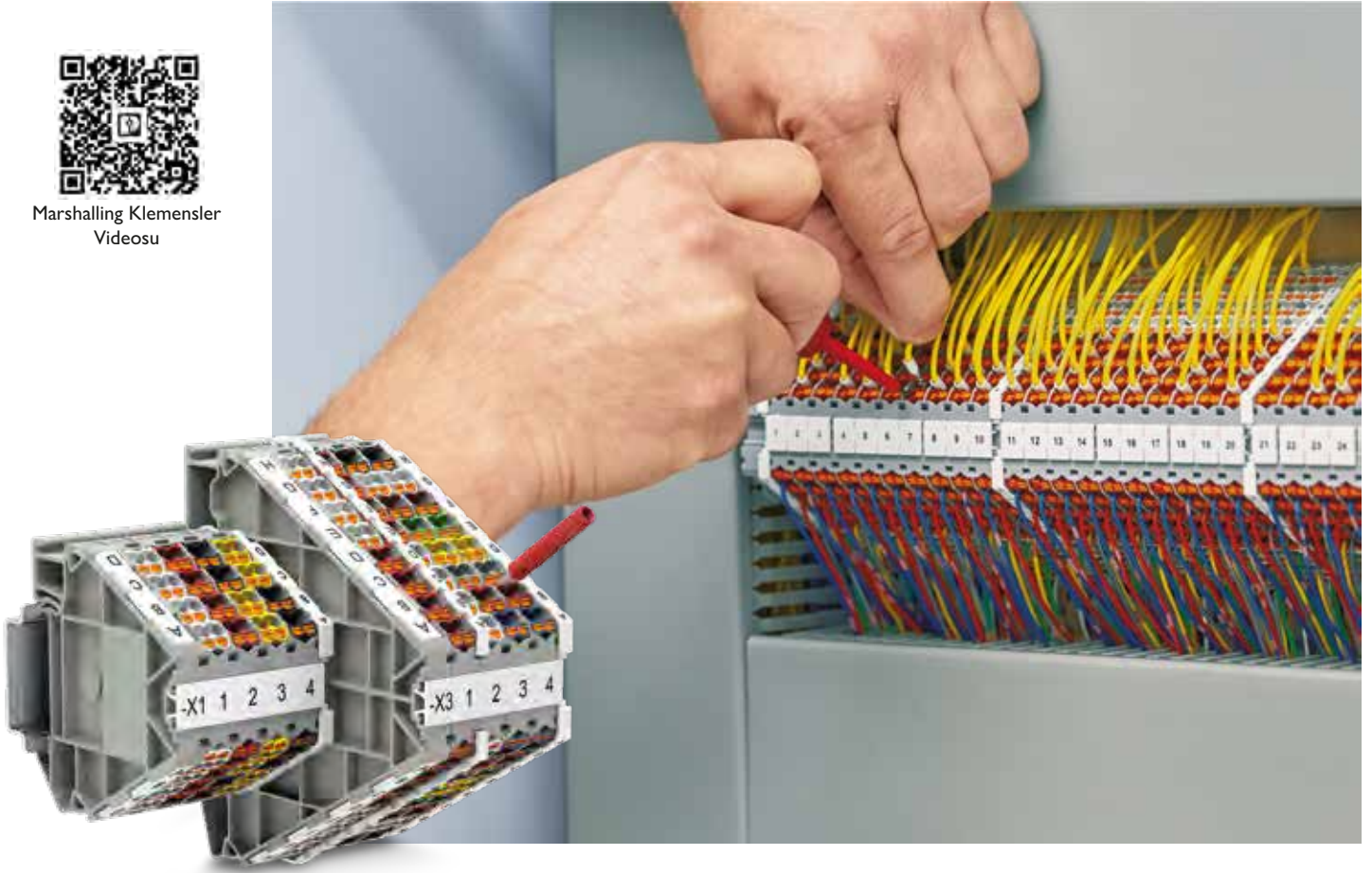
PTRVB 4-PV
