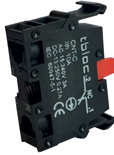
NK/NC Kontakt/Contact
